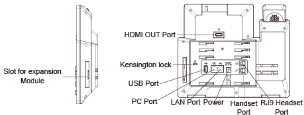
Figure 6: GXV3350 Back / Side View
